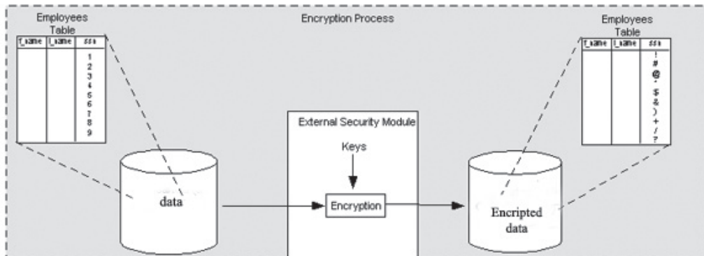
Figure 9.4 – Data Encryption
