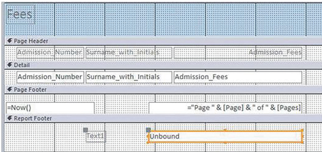
Figure 9.36 - Report plan
