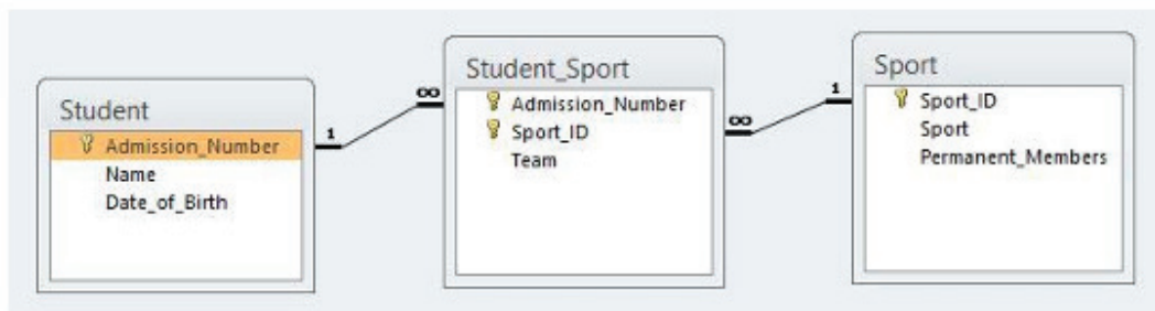
Figure 9.12 - Many-to-Many Relationship
