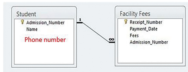
Figure 9.11 - One-to-Many Relationship
