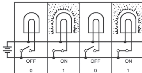
Figure 3.2 – Electronic circuit
