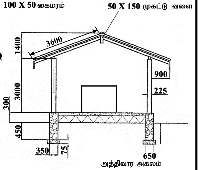
SECTION
